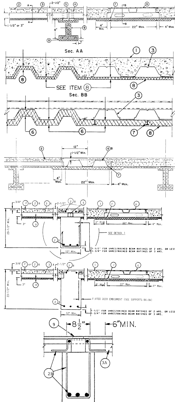
DETAIL I
