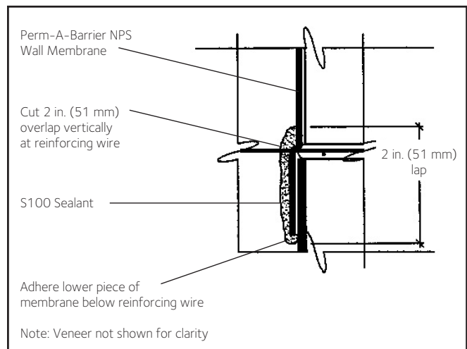
Figure 2: Horizontal Reinforcing
