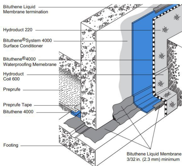
Figure of Bituthene System 4000 Below Grade Application.
