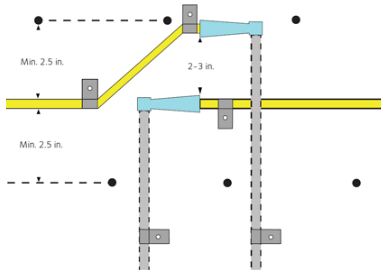
Figure 7. End and beginning of INJECTO® Tube lengths
