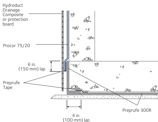
Typical Foundation Waterproofing
