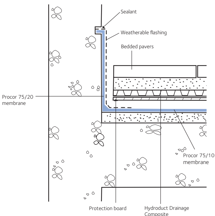
Typical Deck Upright Detail
